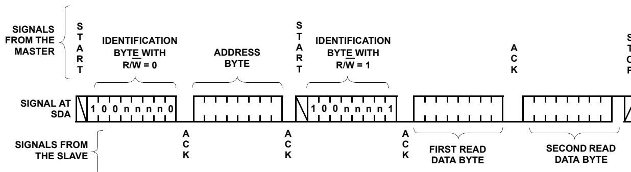
FIGURE 30. READ SEQUENCE (SLAVE ADDRESS SHOWN AS nnnn)
