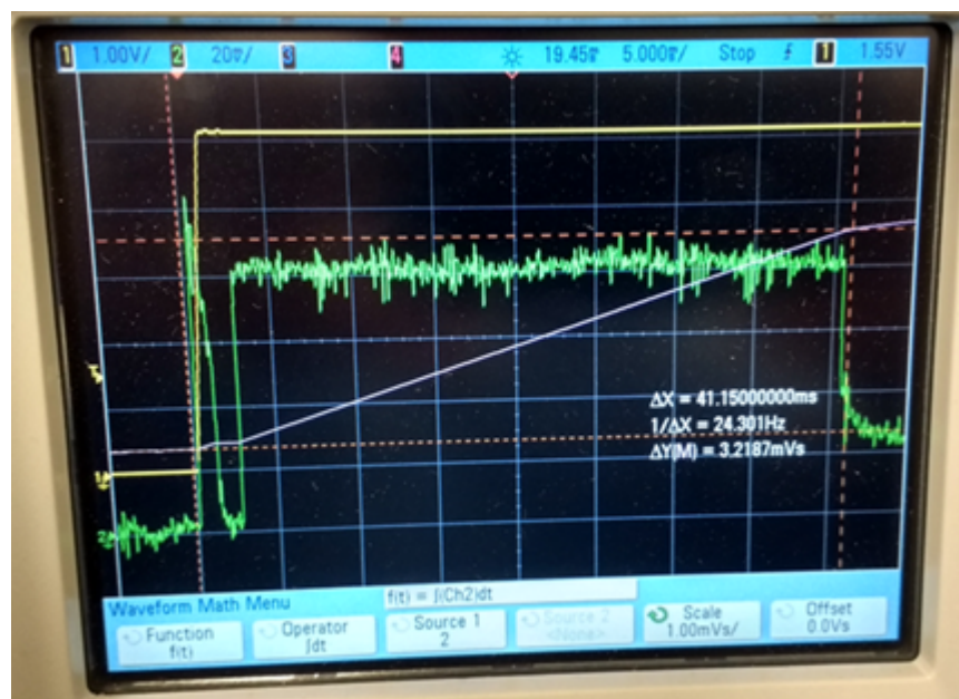
Total Inrush charge of 3.21 mC with 41.1 mS duration
